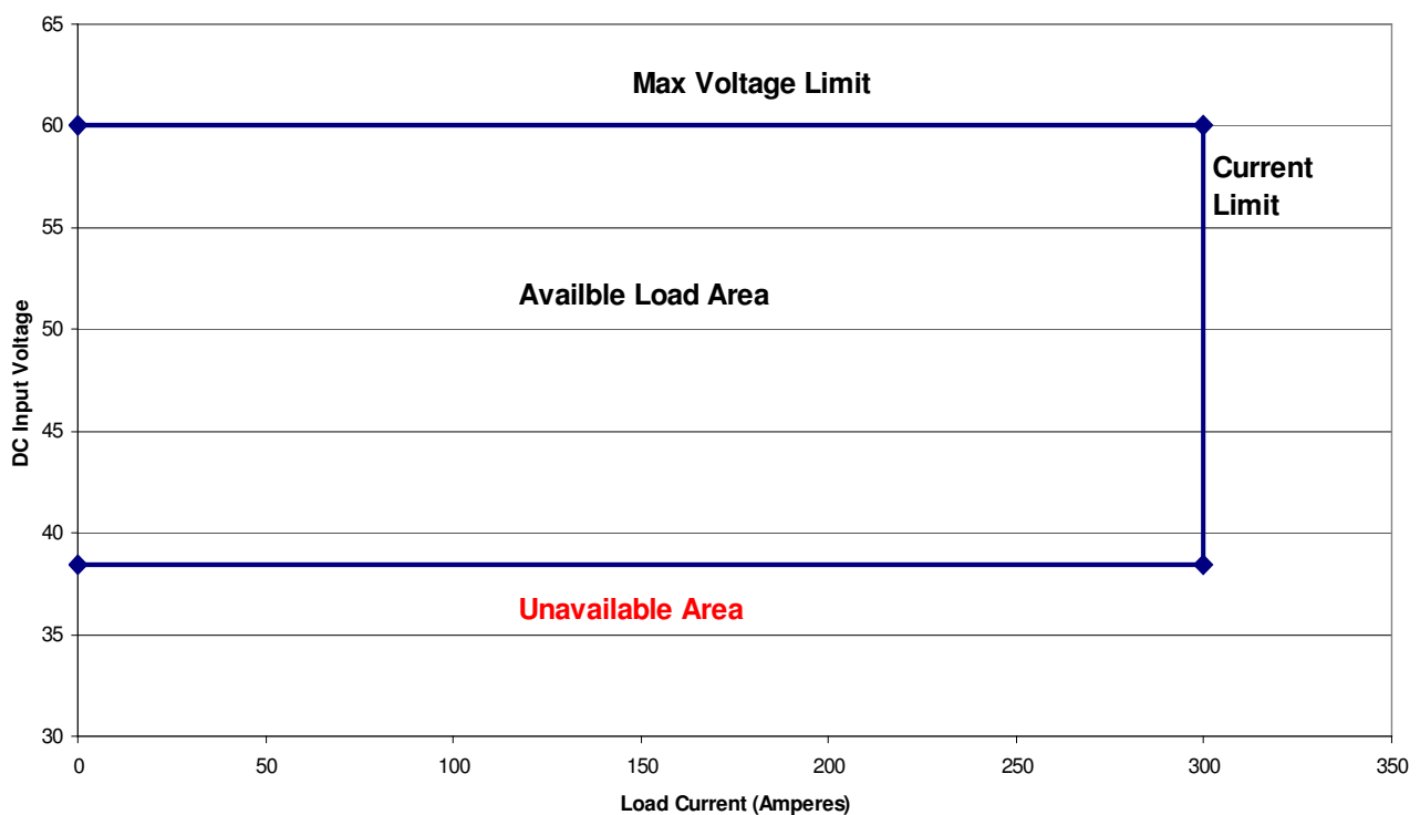
48V / 300A Model Operating Area
